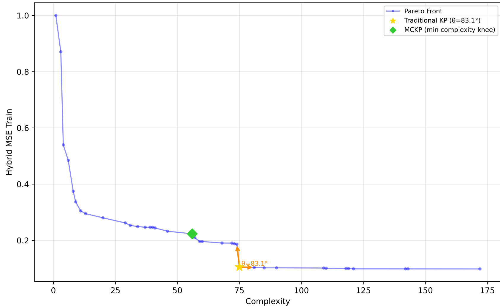
637_fri_c1_500_50 - Run 7 - SVP - Hybrid MSE Train \lambda_1=0.00, \lambda_2=0.00, \lambda_3=0.00 | Difficulty: 1.00 | Method: hmr
