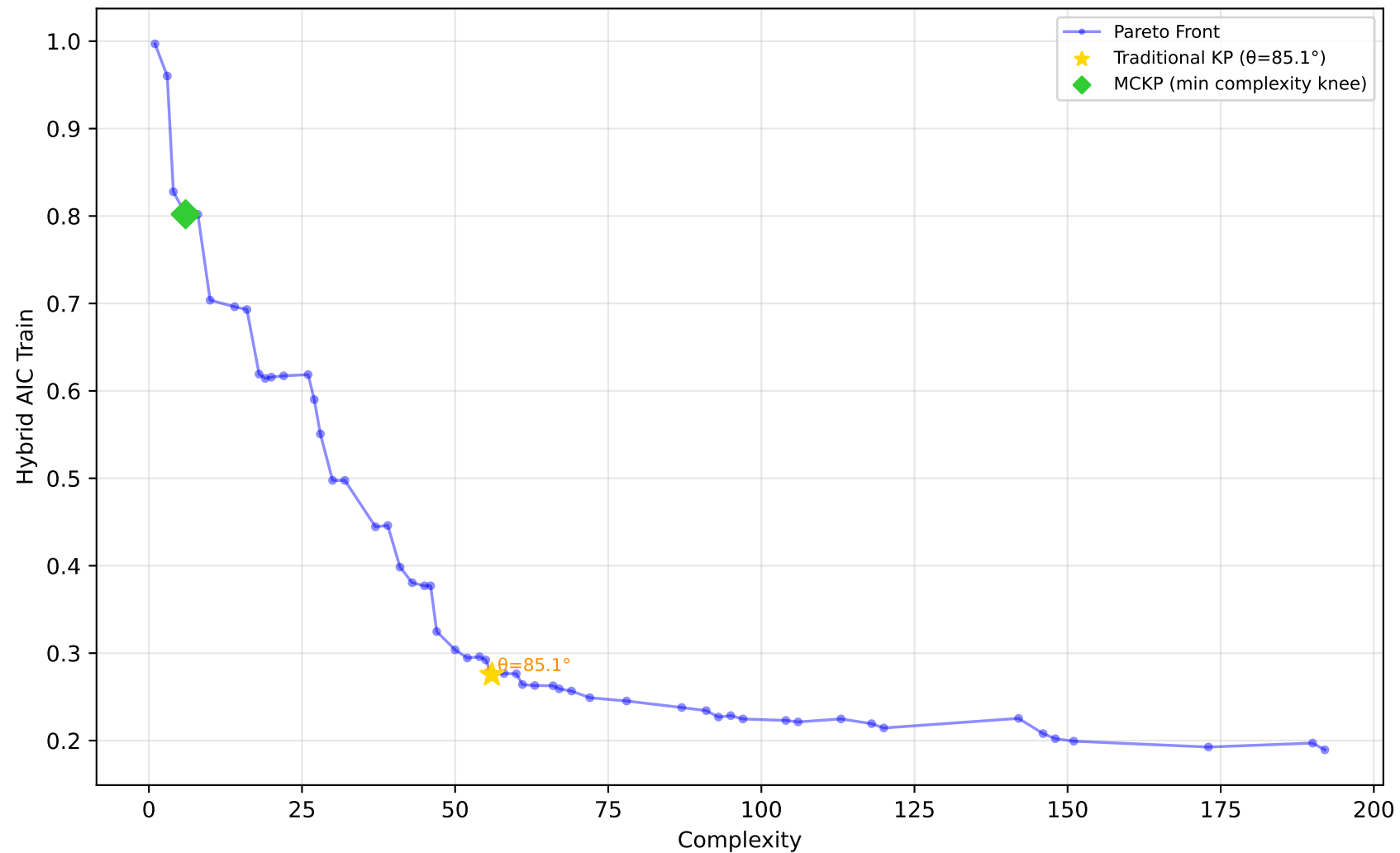
637_fri_c1_500_50 - Run 8 - MVP - Hybrid AIC Train \lambda_1=0.00, \lambda_2=0.50, \lambda_3=0.00 | Difficulty: 1.00 | Method: hmr
