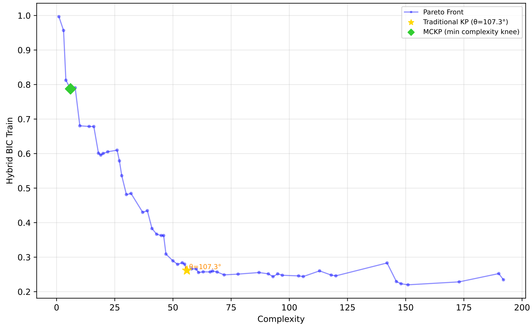
637_fri_c1_500_50 - Run 8 - MVP - Hybrid BIC Train \lambda_1=0.00, \lambda_2=0.50, \lambda_3=0.00 | Difficulty: 1.00 | Method: hmr
