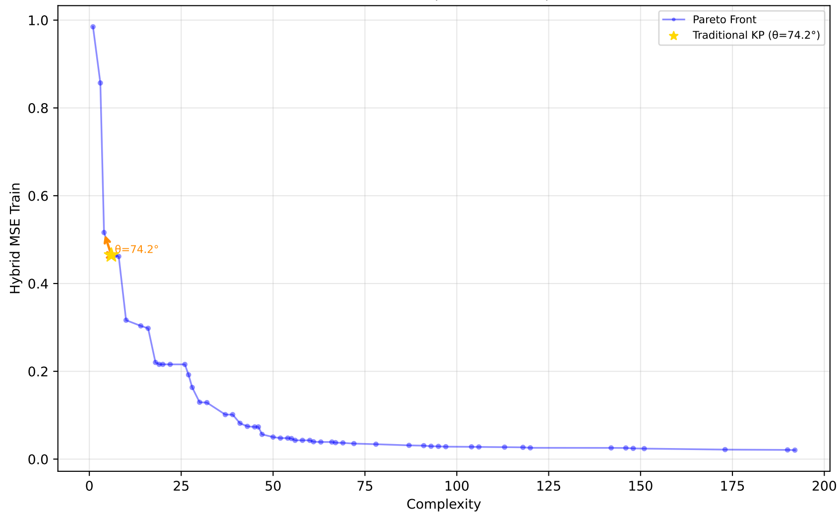
637_fri_c1_500_50 - Run 8 - MVP - Hybrid MSE Train \lambda_1=0.00, \lambda_2=0.50, \lambda_3=0.00 | Difficulty: 1.00 | Method: hmr
