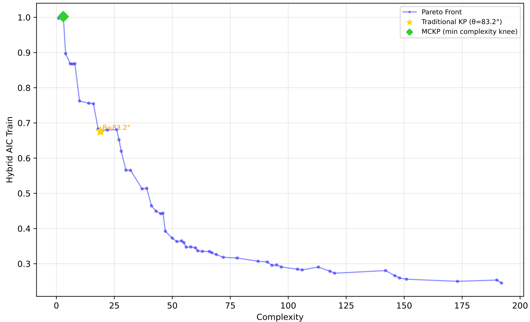
637_fri_c1_500_50 - Run 8 - SVP - Hybrid AIC Train \lambda_1=0.10 , \lambda_2=0.00 , \lambda_3=0.20 | Difficulty: 1.00 | Method: hmr
