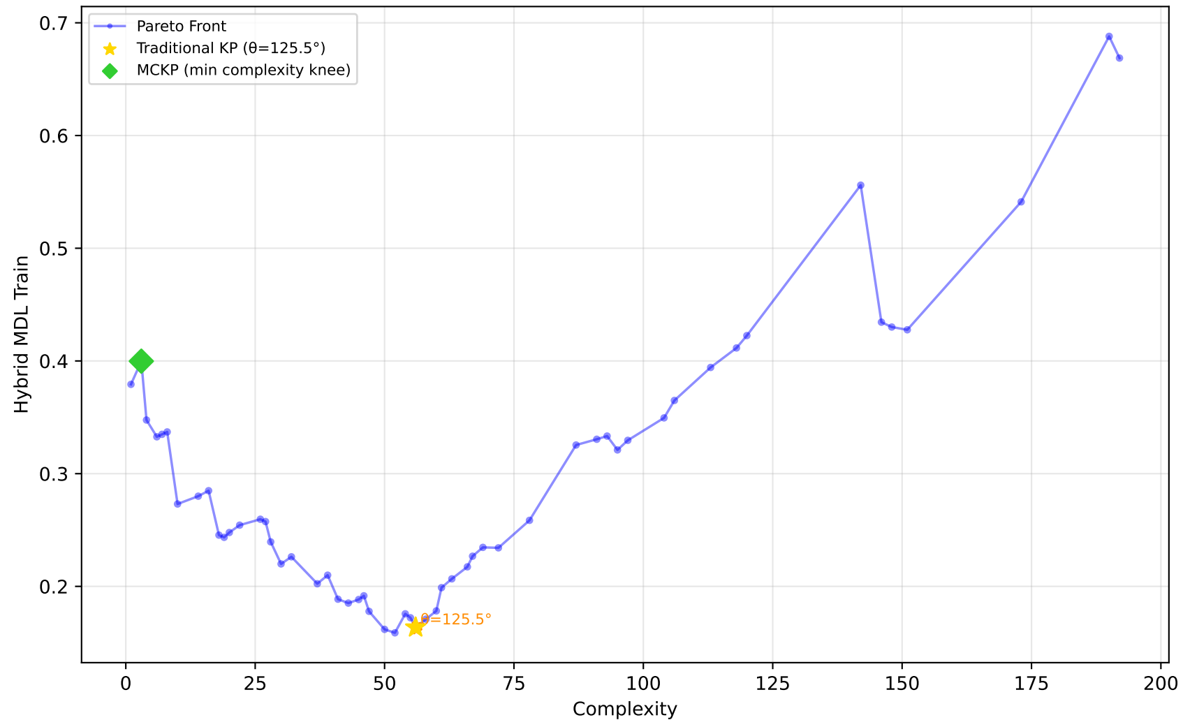
637_fri_c1_500_50 - Run 8 - SVP - Hybrid MDL Train \lambda_1=0.10, \lambda_2=0.00, \bar{\lambda}_3=0.20 | Difficulty: 1.00 | Method: hmr
