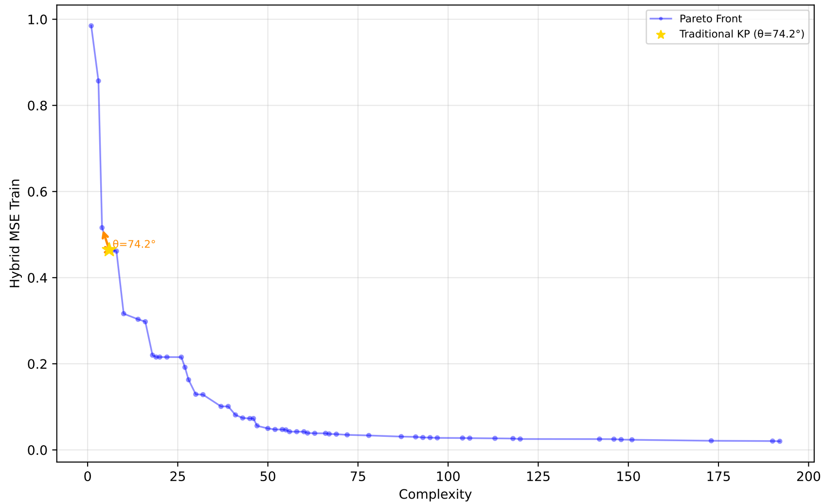
637_fri_c1_500_50 - Run 8 - SVP - Hybrid MSE Train \lambda_1=0.00, \lambda_2=0.00, \lambda_3=0.00 | Difficulty: 1.00 | Method: hmr
