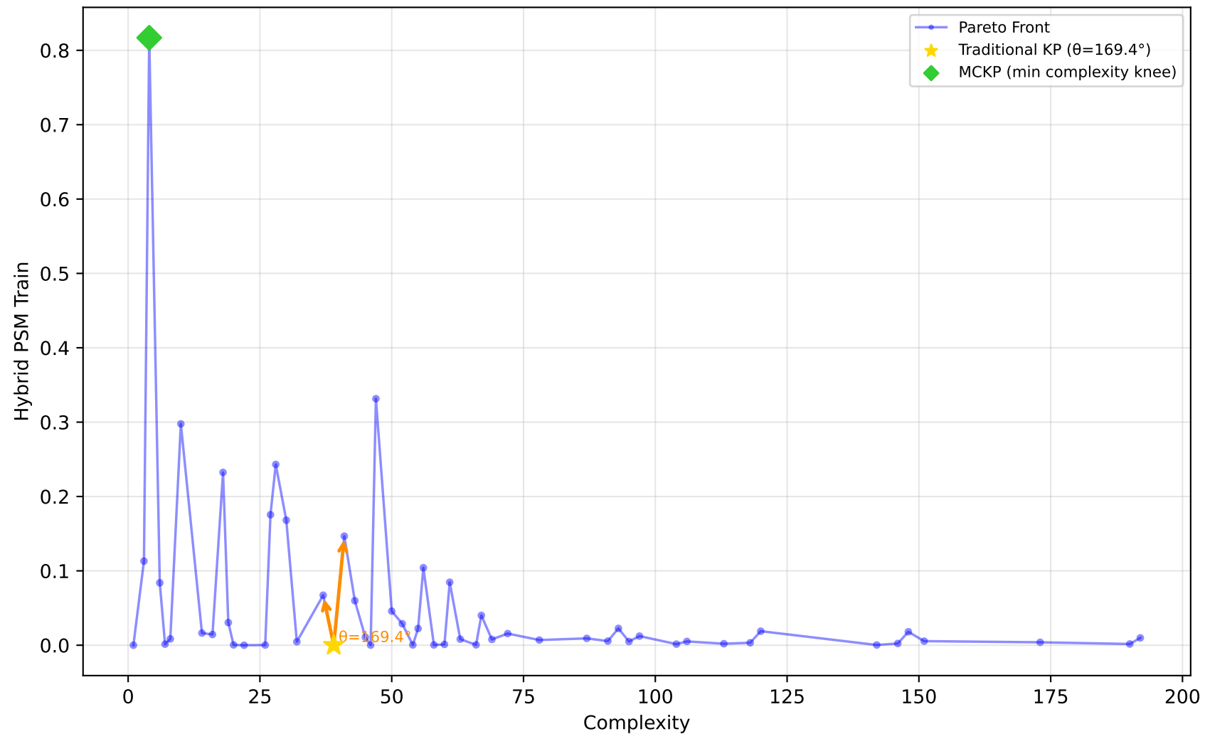
637_fri_c1_500_50 - Run 8 - SVP - Hybrid PSM Train \lambda_1=0.00, \lambda_2=0.00, \lambda_3=0.00 | Difficulty: 1.00 | Method: hmr
