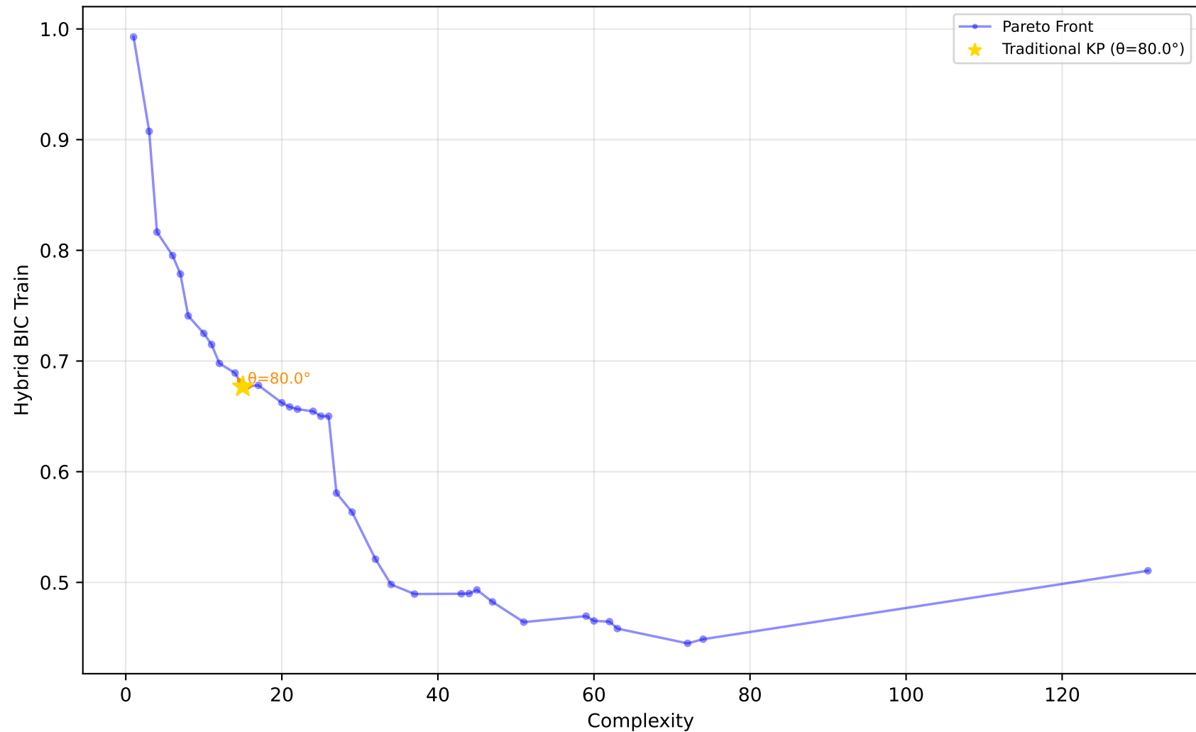
637_fri_c1_500_50 - Run 9 - MVP - Hybrid BIC Train \lambda_1=0.00, \lambda_2=0.50, \lambda_3=0.00 | Difficulty: 1.00 | Method: hmr
