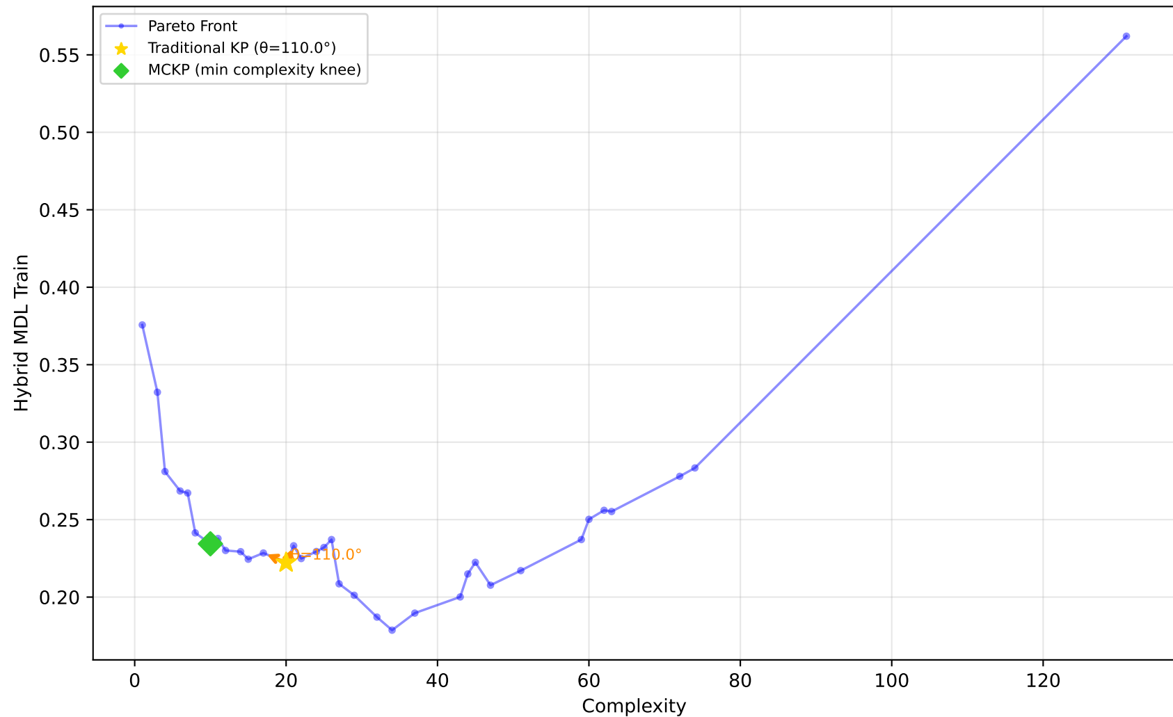
637_fri_c1_500_50 - Run 9 - MVP - Hybrid MDL Train \lambda_1=0.00, \lambda_2=0.50, \lambda_3=0.00 | Difficulty: 1.00 | Method: hmr
