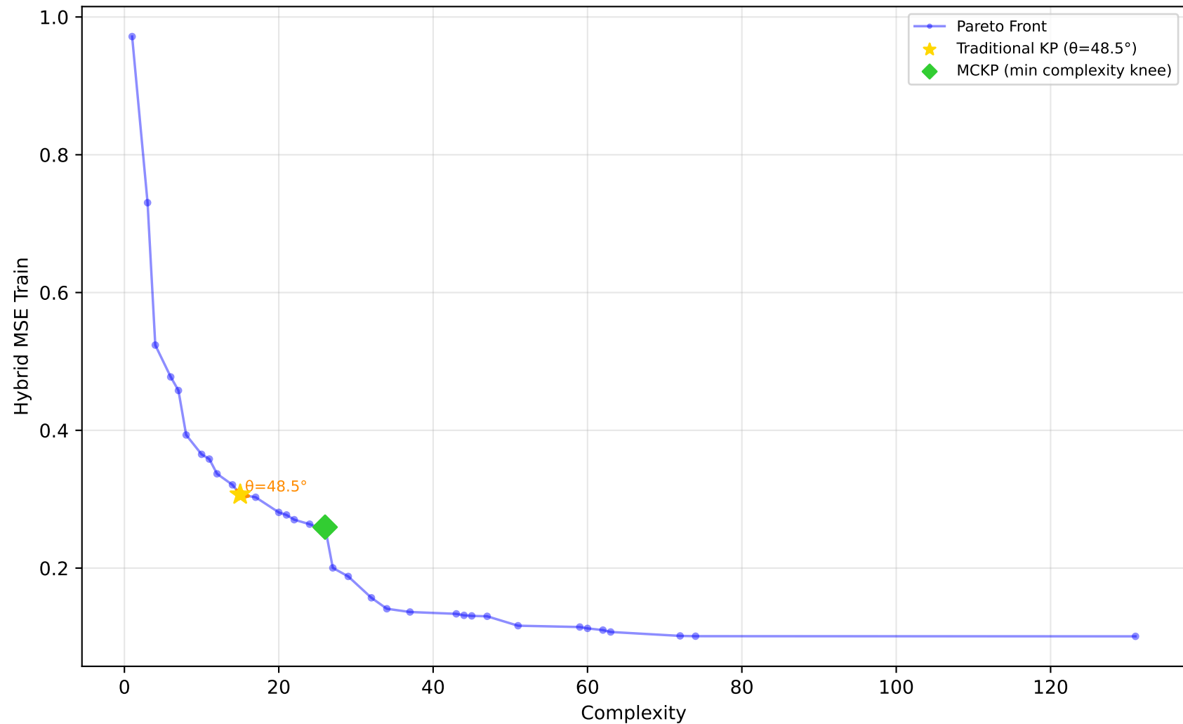
637_fri_c1_500_50 - Run 9 - MVP - Hybrid MSE Train \lambda_1=0.00, \lambda_2=0.50, \lambda_3=0.00 | Difficulty: 1.00 | Method: hmr
