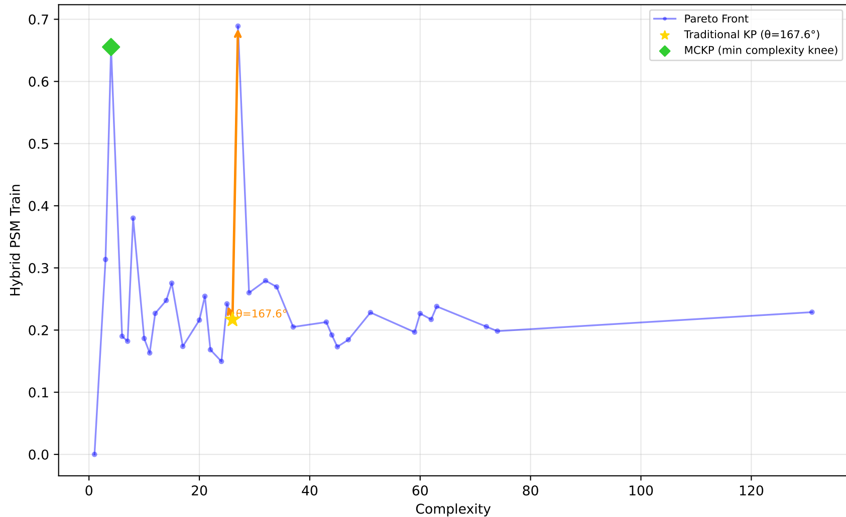
637_fri_c1_500_50 - Run 9 - MVP - Hybrid PSM Train \lambda_1=0.10, \lambda_2=0.00, \lambda_3=1.00 | Difficulty: 1.00 | Method: hmr
