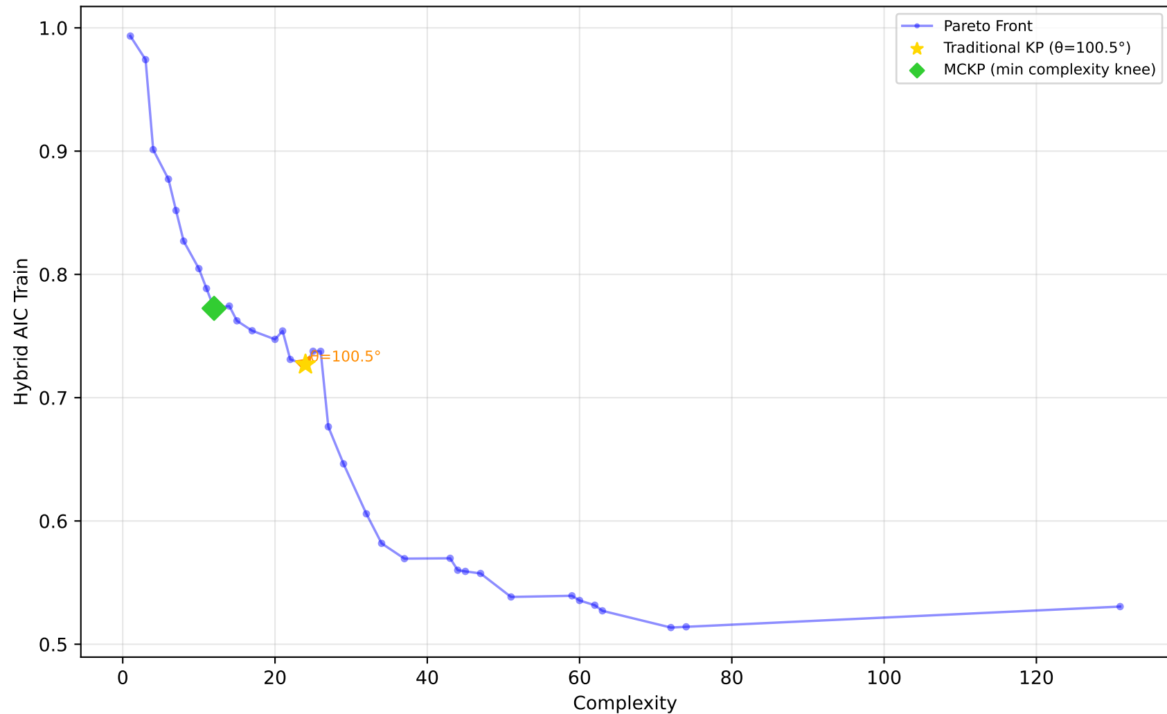
637_fri_c1_500_50 - Run 9 - SVP - Hybrid AIC Train \lambda_1=0.10, \lambda_2=0.00, \lambda_3=0.20 | Difficulty: 1.00 | Method: hmr
