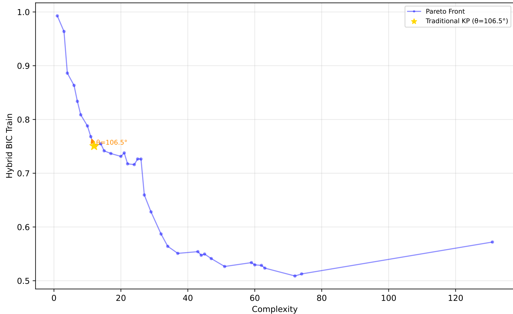
637_fri_c1_500_50 - Run 9 - SVP - Hybrid BIC Train \lambda_1=0.10, \lambda_2=0.00, \lambda_3=0.20 | Difficulty: 1.00 | Method: hmr
