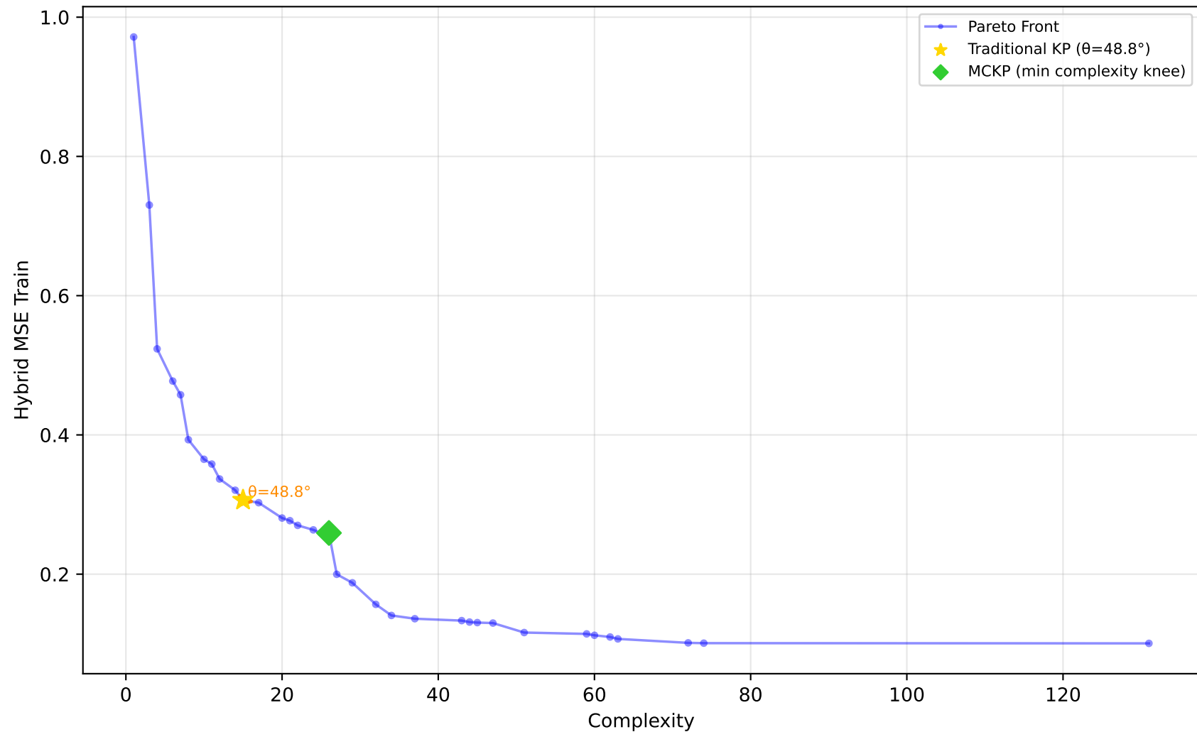
637_fri_c1_500_50 - Run 9 - SVP - Hybrid MSE Train \lambda_1=0.00, \lambda_2=0.00, \lambda_3=0.00 | Difficulty: 1.00 | Method: hmr
