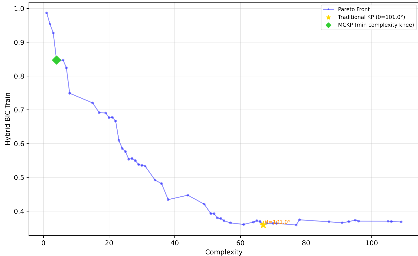
584_fri_c4_500_25 - Run 10 - MVP - Hybrid BIC Train \lambda_1=0.00, \lambda_2=0.00, \lambda_3=0.00 | Difficulty: 1.00 | Method: hmr
