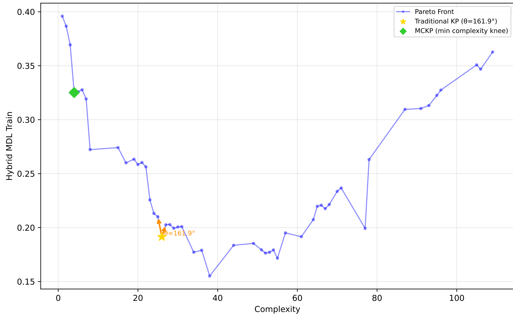
584_fri_c4_500_25 - Run 10 - MVP - Hybrid MDL Train \lambda_1=0.10 , \lambda_2=0.00 , \lambda_3=0.00 | Difficulty: 1.00 | Method: hmr
