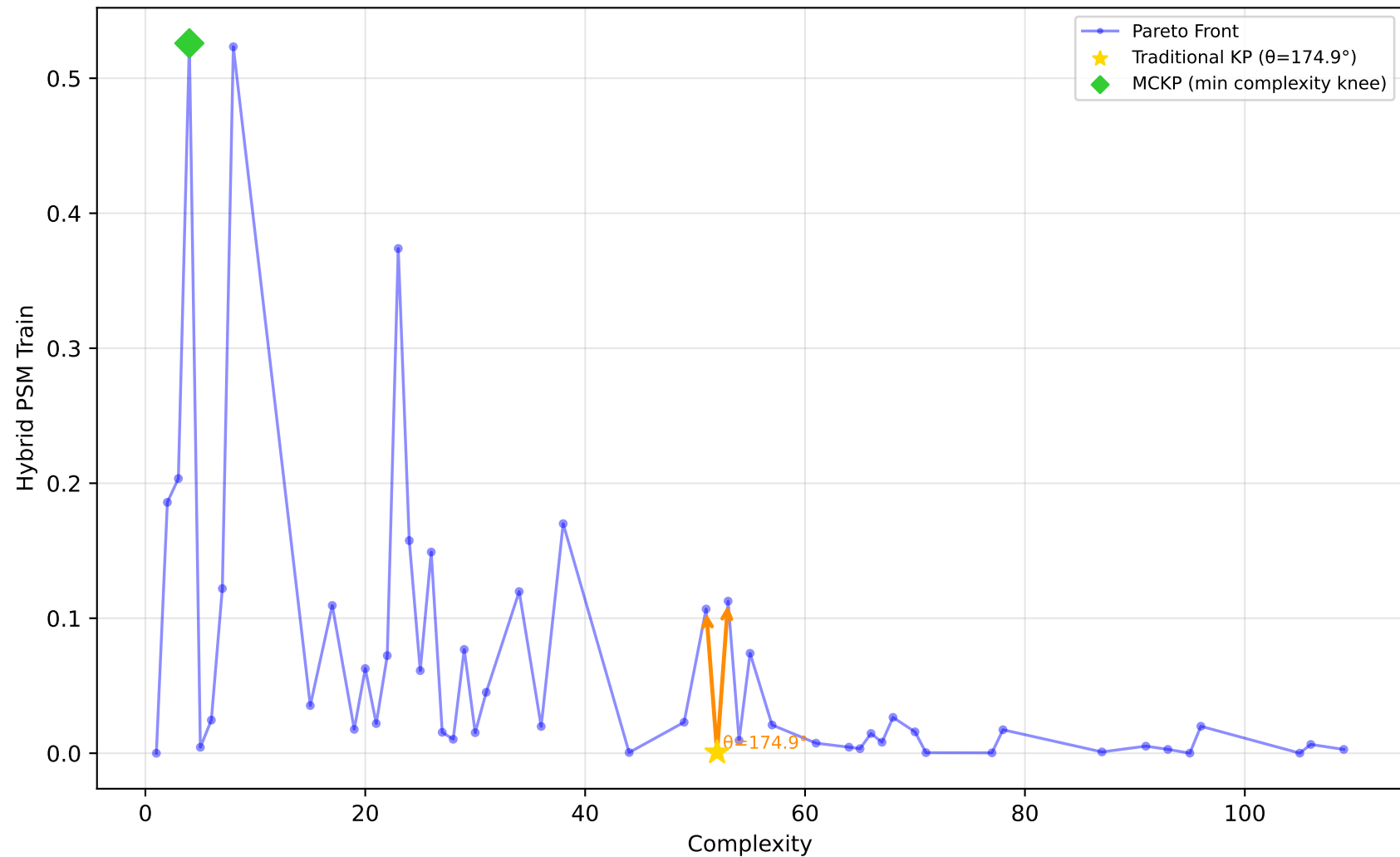
584_fri_c4_500_25 - Run 10 - MVP - Hybrid PSM Train \lambda_1=0.00, \lambda_2=0.00, \lambda_3=0.00 | Difficulty: 1.00 | Method: hmr
