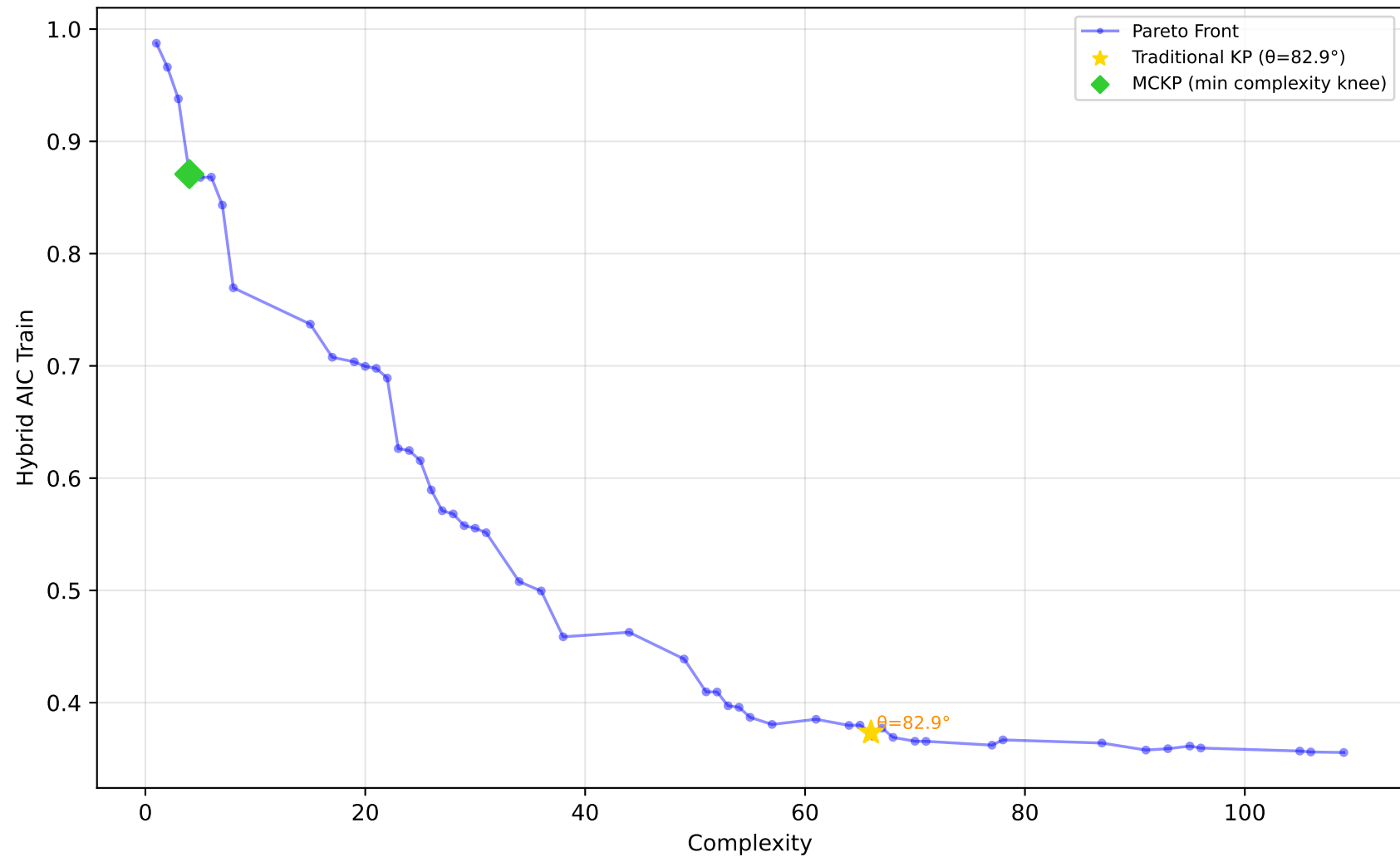
584_fri_c4_500_25 - Run 10 - SVP - Hybrid AIC Train \lambda_1=0.10, \lambda_2=0.40, \lambda_3=0.00 | Difficulty: 1.00 | Method: hmr
