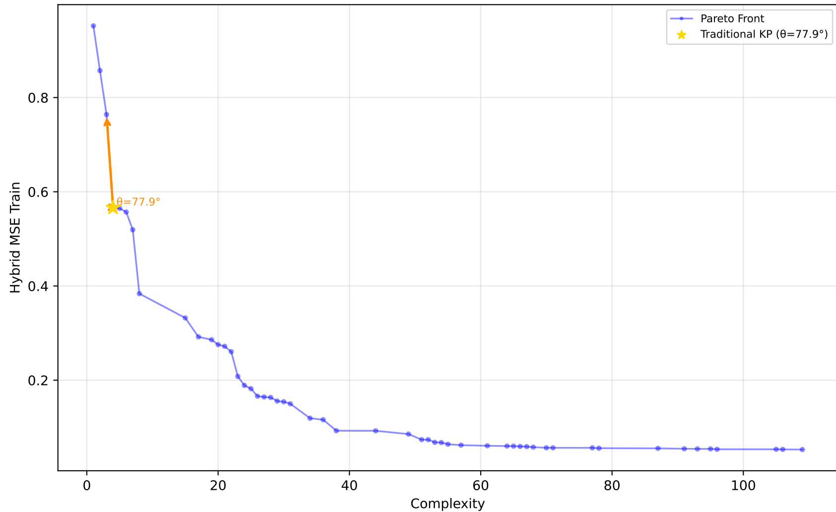
584_fri_c4_500_25 - Run 10 - SVP - Hybrid MSE Train \lambda_1=0.00, \lambda_2=0.00, \lambda_3=0.00 | Difficulty: 1.00 | Method: hmr
