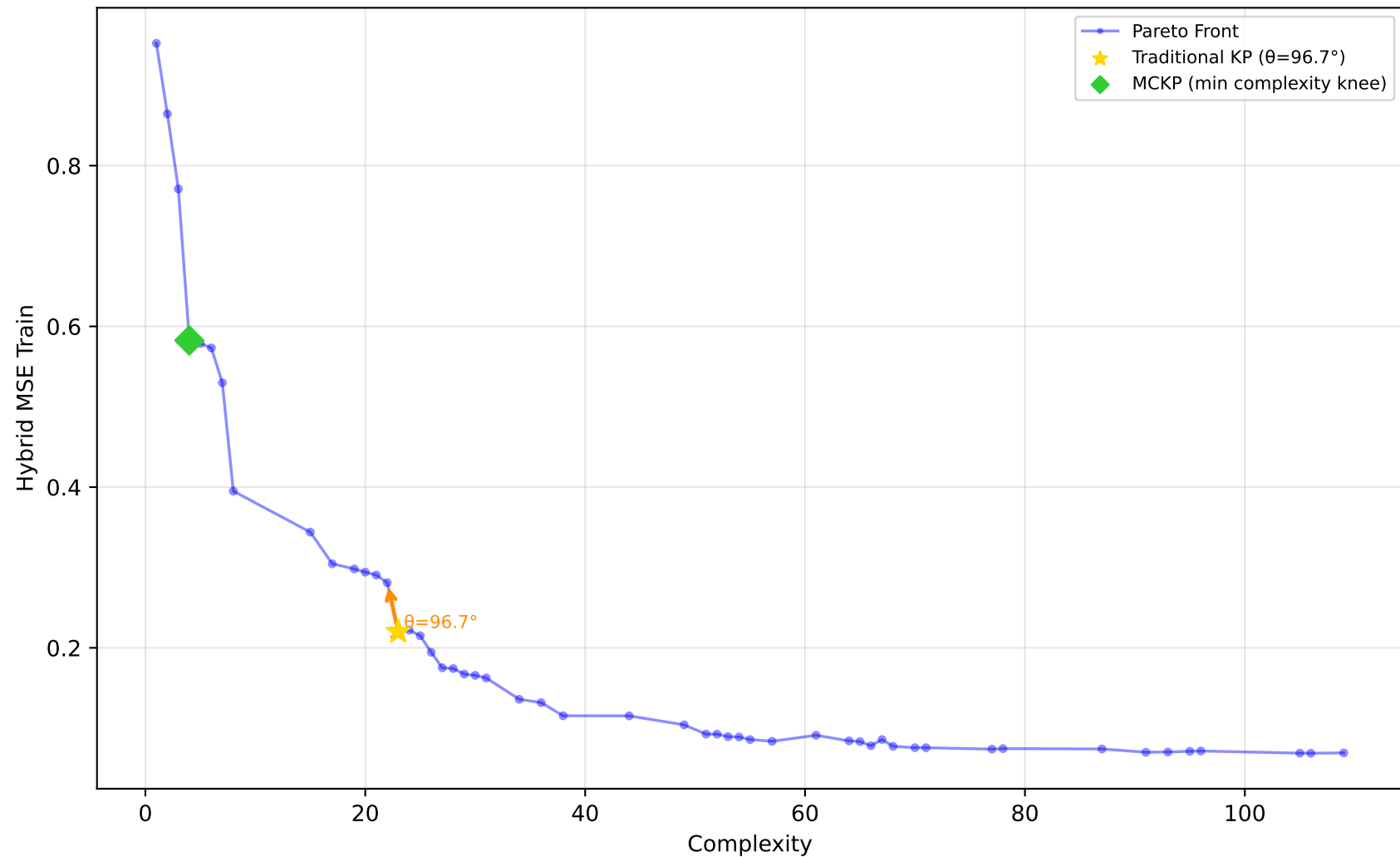
584_fri_c4_500_25 - Run 10 - SVP - Hybrid MSE Train \lambda_1=0.10, \lambda_2=0.40, \lambda_3=0.00 | Difficulty: 1.00 | Method: hmr
