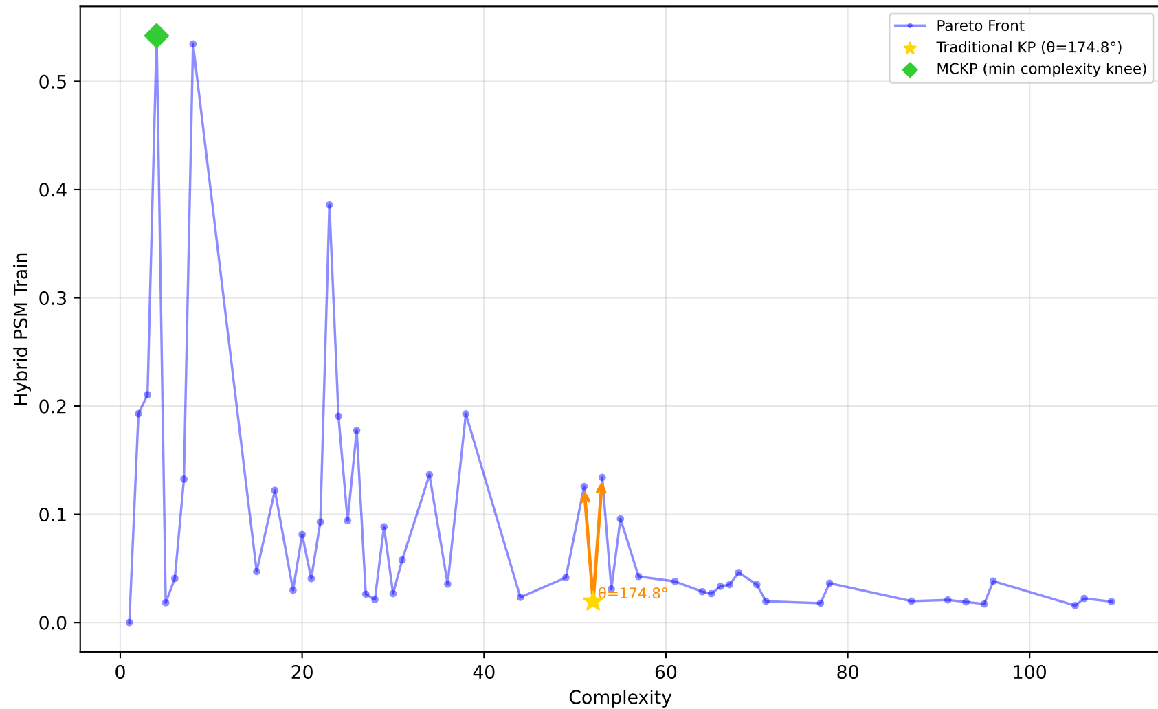
584_fri_c4_500_25 - Run 10 - SVP - Hybrid PSM Train \lambda_1=0.10, \lambda_2=0.40, \lambda_3=0.00 | Difficulty: 1.00 | Method: hmr
