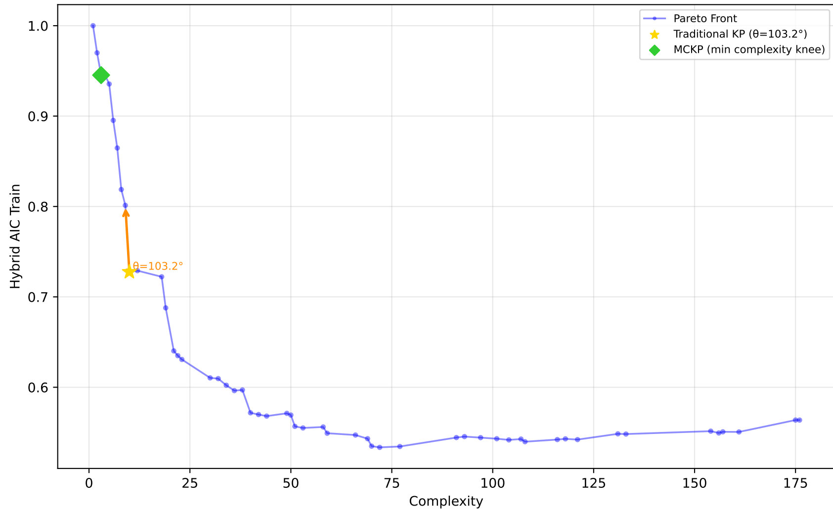
584_fri_c4_500_25 - Run 11 - MVP - Hybrid AIC Train \lambda_1=0.10, \lambda_2=0.00, \lambda_3=0.00 | Difficulty: 1.00 | Method: hmr
