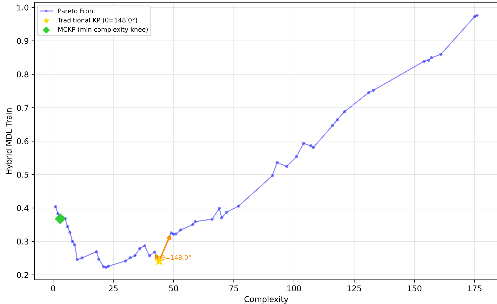
584_fri_c4_500_25 - Run 11 - MVP - Hybrid MDL Train \lambda_1=0.00, \bar{\lambda}_2=0.00, \lambda_3=0.00 | Difficulty: 1.00 | Method: hmr
