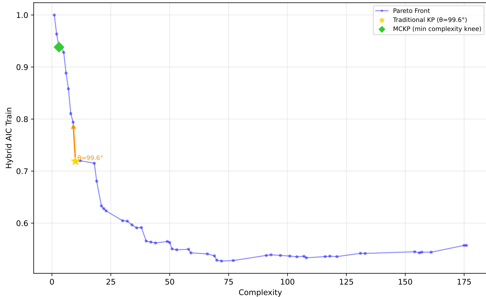
584_fri_c4_500_25 - Run 11 - SVP - Hybrid AIC Train \lambda_1=0.00, \lambda_2=0.00, \lambda_3=0.00 | Difficulty: 1.00 | Method: hmr
