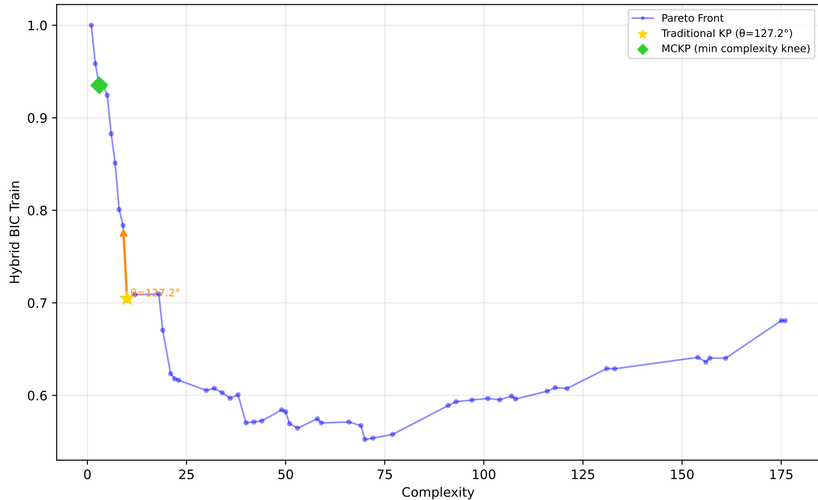
584_fri_c4_500_25 - Run 11 - SVP - Hybrid BIC Train \lambda_1=0.00, \lambda_2=0.00, \lambda_3=0.00 | Difficulty: 1.00 | Method: hmr
