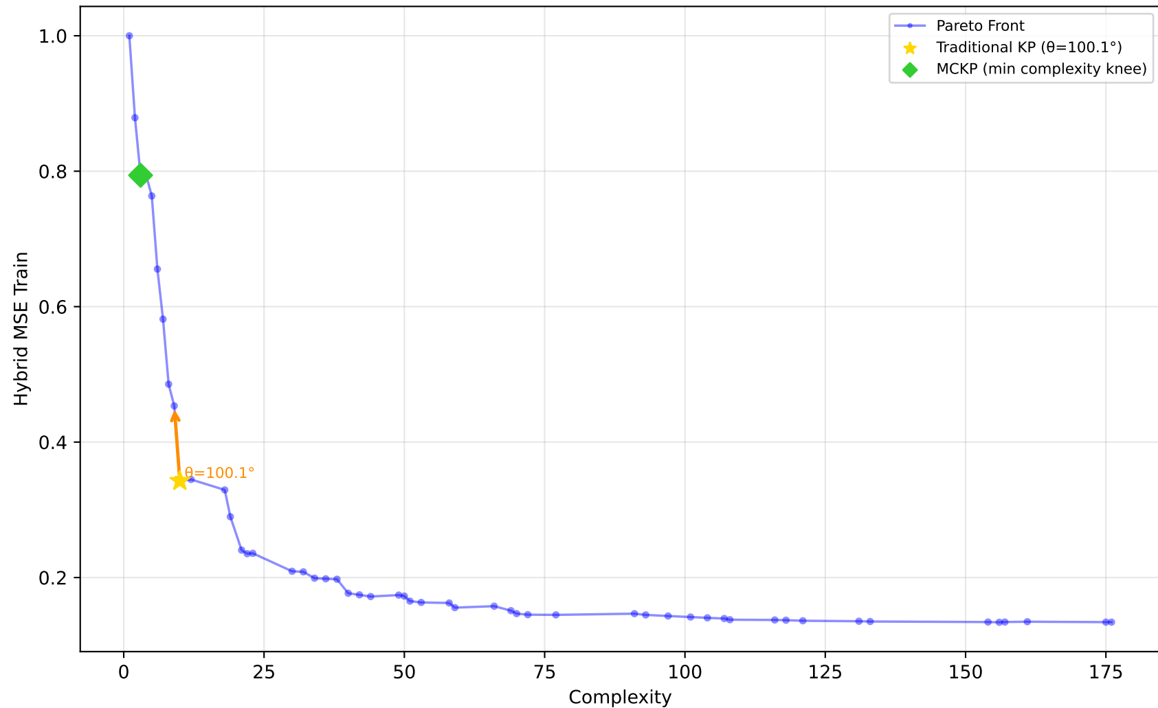
584_fri_c4_500_25 - Run 11 - SVP - Hybrid MSE Train \lambda_1=0.10, \lambda_2=0.40, \lambda_3=0.00 | Difficulty: 1.00 | Method: hmr
