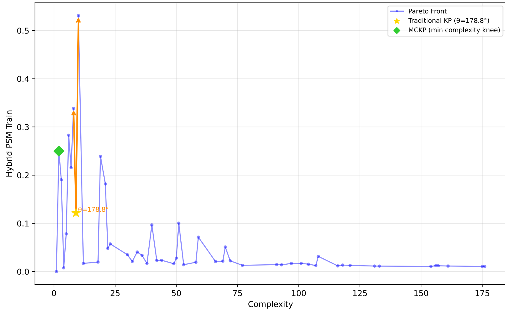
584_fri_c4_500_25 - Run 11 - SVP - Hybrid PSM Train \lambda_1=0.10, \lambda_2=0.40, \lambda_3=0.00 | Difficulty: 1.00 | Method: hmr
