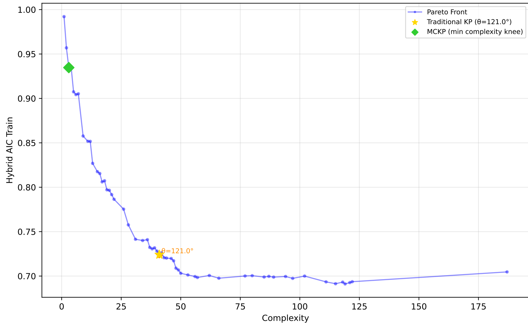
584_fri_c4_500_25 - Run 12 - MVP - Hybrid AIC Train \lambda_1=0.10 , \lambda_2=0.00 , \lambda_3=0.00 | Difficulty: 1.00 | Method: hmr
