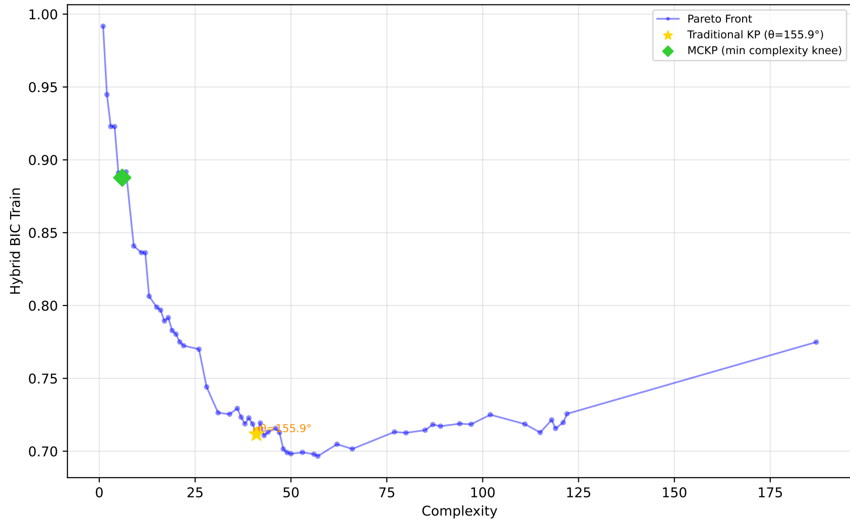
584_fri_c4_500_25 - Run 12 - MVP - Hybrid BIC Train \lambda_1=0.00, \lambda_2=0.00, \lambda_3=0.00 | Difficulty: 1.00 | Method: hmr
