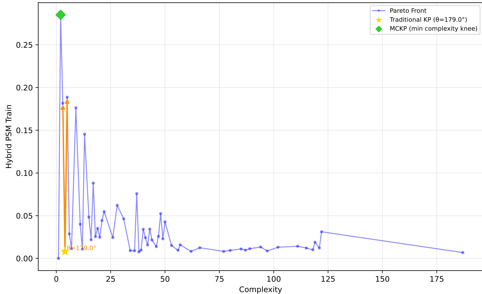
584_fri_c4_500_25 - Run 12 - MVP - Hybrid PSM Train \lambda_1=0.10, \lambda_2=0.00, \lambda_3=0.00 | Difficulty: 1.00 | Method: hmr
