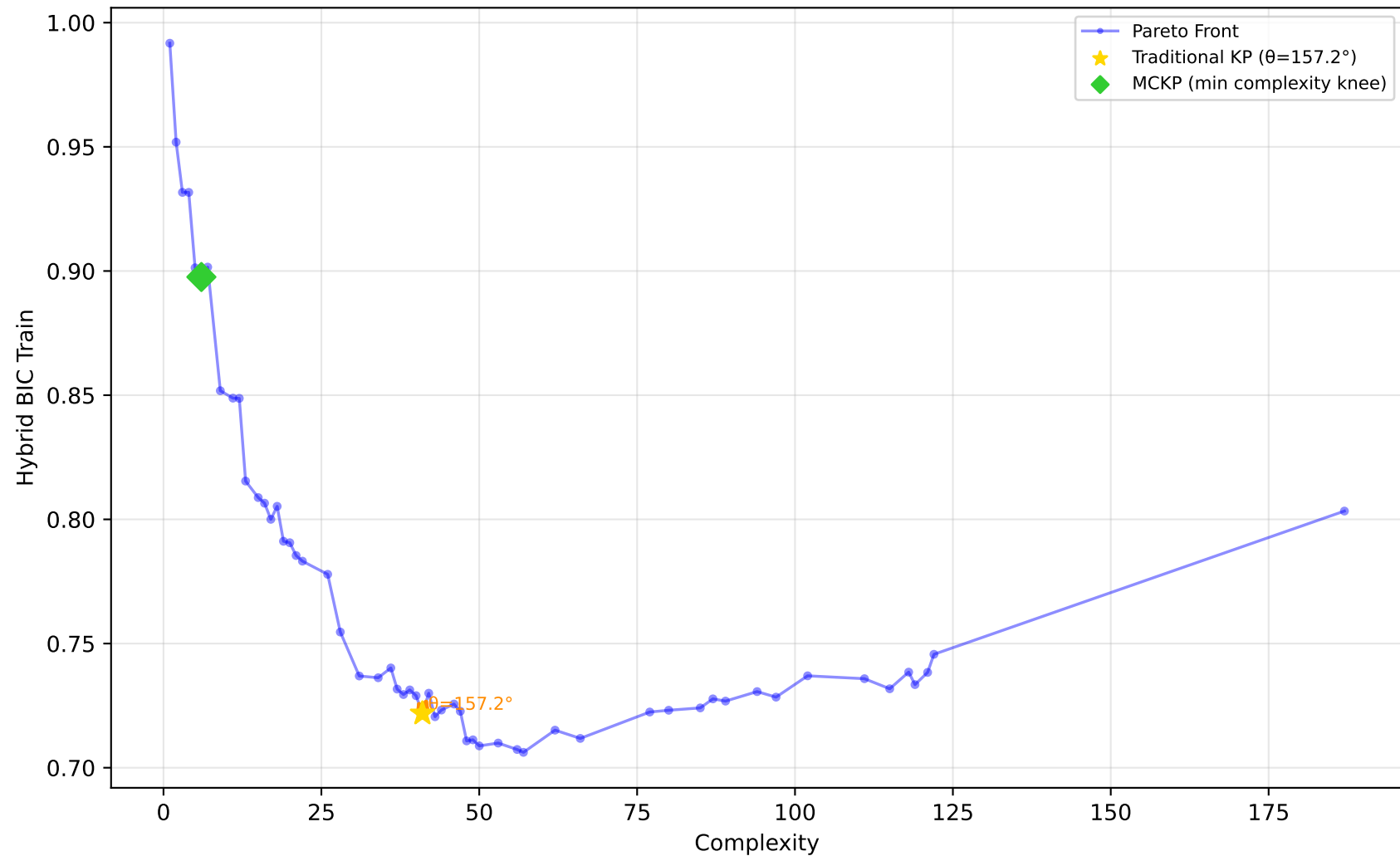
584_fri_c4_500_25 - Run 12 - SVP - Hybrid BIC Train \lambda_1=0.10, \lambda_2=0.40, \lambda_3=0.00 | Difficulty: 1.00 | Method: hmr
