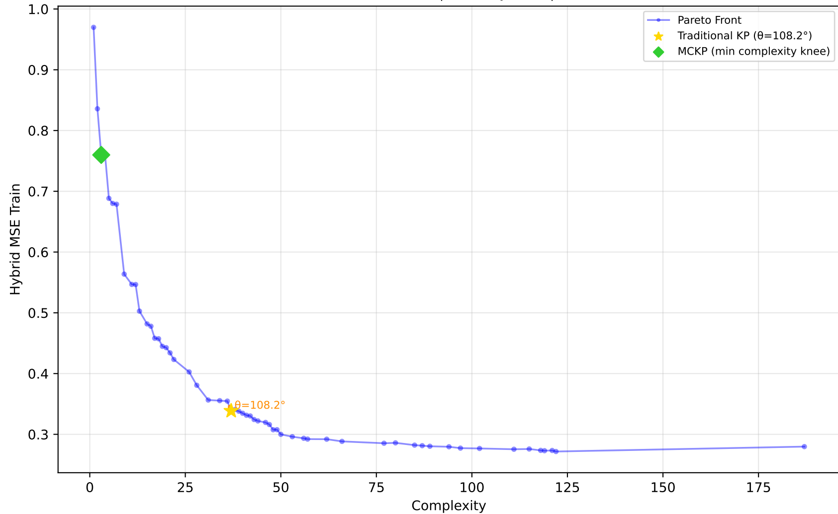
584_fri_c4_500_25 - Run 12 - SVP - Hybrid MSE Train \lambda_1=0.10, \lambda_2=0.40, \lambda_3=0.00 | Difficulty: 1.00 | Method: hmr
