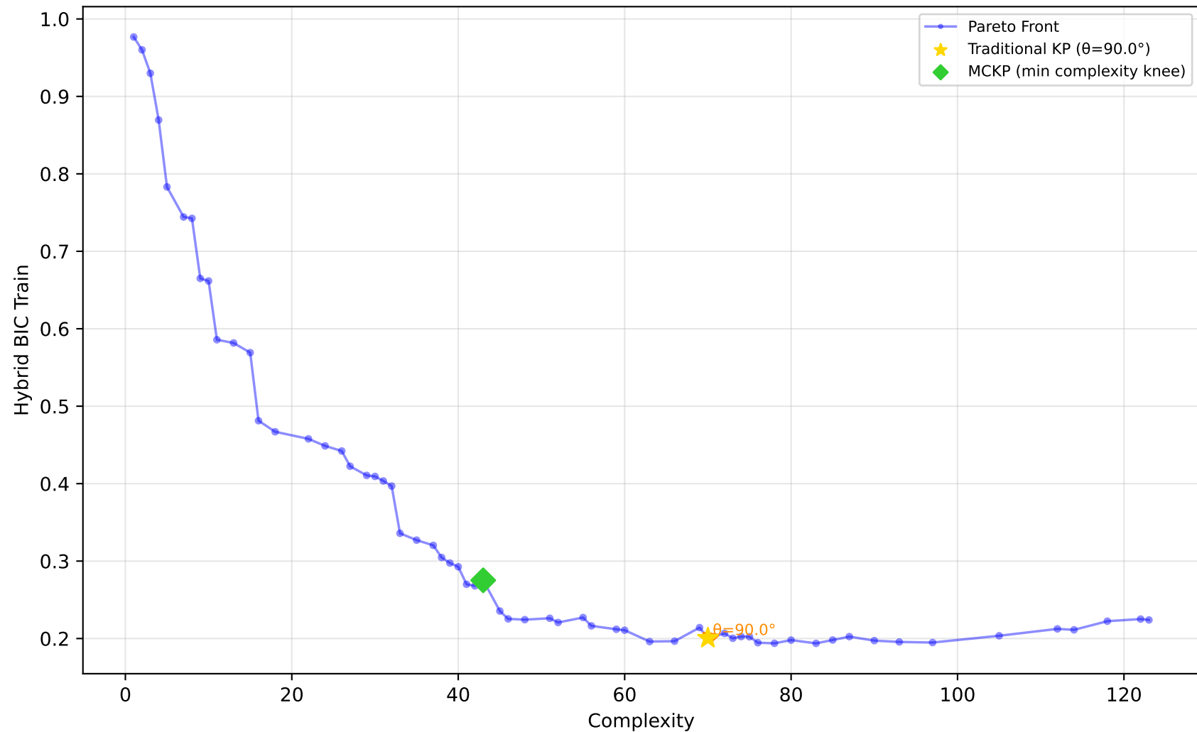
584_fri_c4_500_25 - Run 13 - MVP - Hybrid BIC Train \lambda_1=0.10, \lambda_2=0.00, \lambda_3=0.00 | Difficulty: 1.00 | Method: hmr
