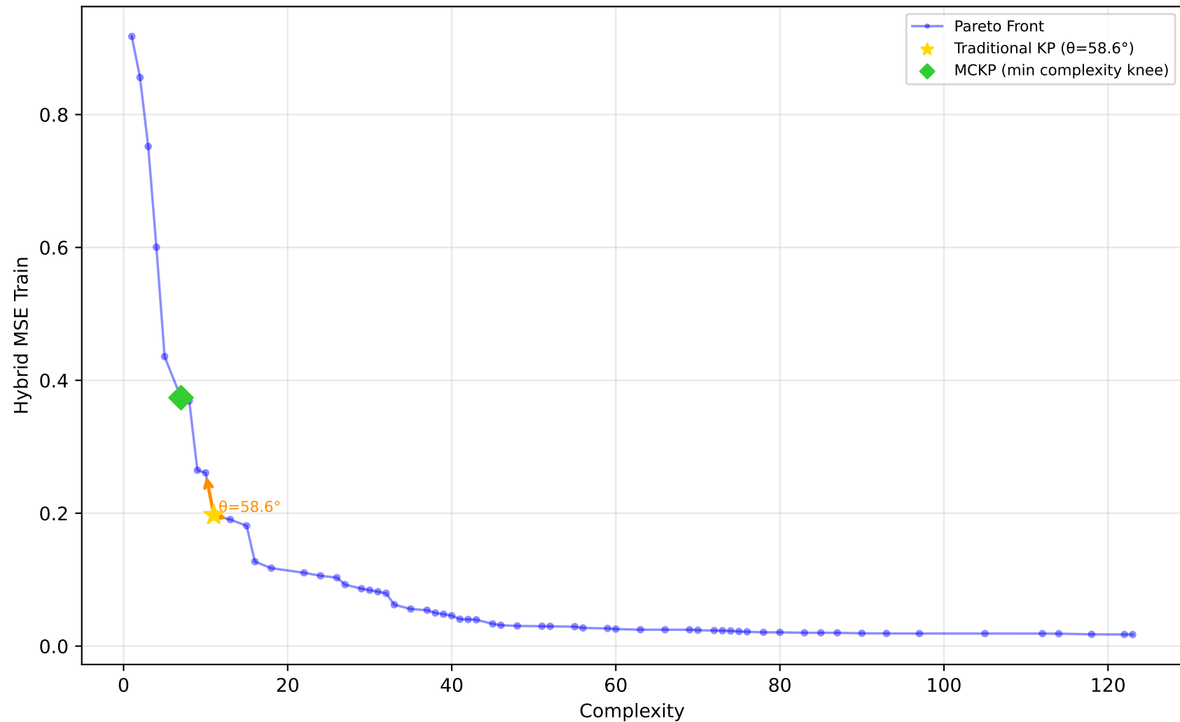
584_fri_c4_500_25 - Run 13 - MVP - Hybrid MSE Train \lambda_1=0.00, \lambda_2=0.00, \lambda_3=0.00 | Difficulty: 1.00 | Method: hmr
