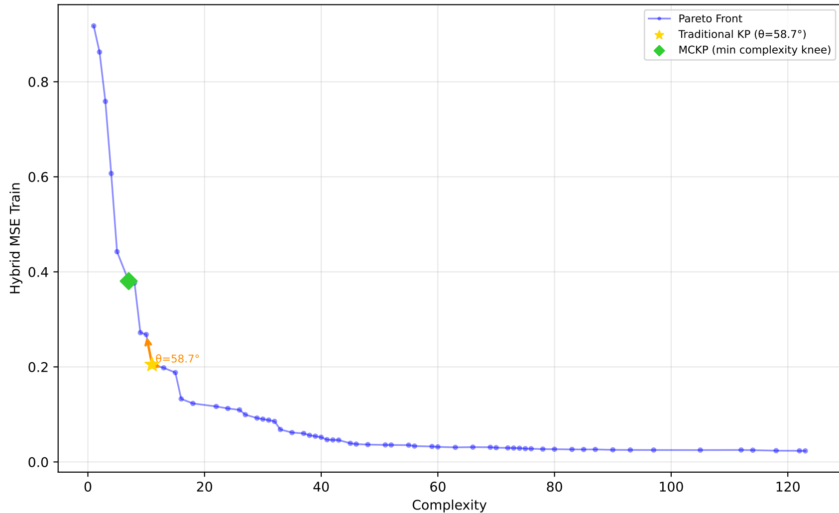
584_fri_c4_500_25 - Run 13 - MVP - Hybrid MSE Train \lambda_1=0.10, \lambda_2=0.00, \lambda_3=0.00 | Difficulty: 1.00 | Method: hmr
