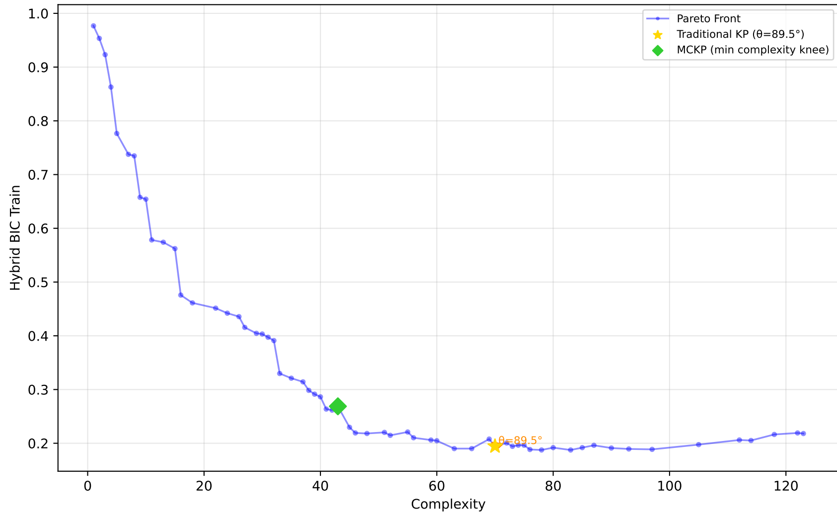
584_fri_c4_500_25 - Run 13 - SVP - Hybrid BIC Train \lambda_1=0.00, \lambda_2=0.00, \lambda_3=0.00 | Difficulty: 1.00 | Method: hmr
