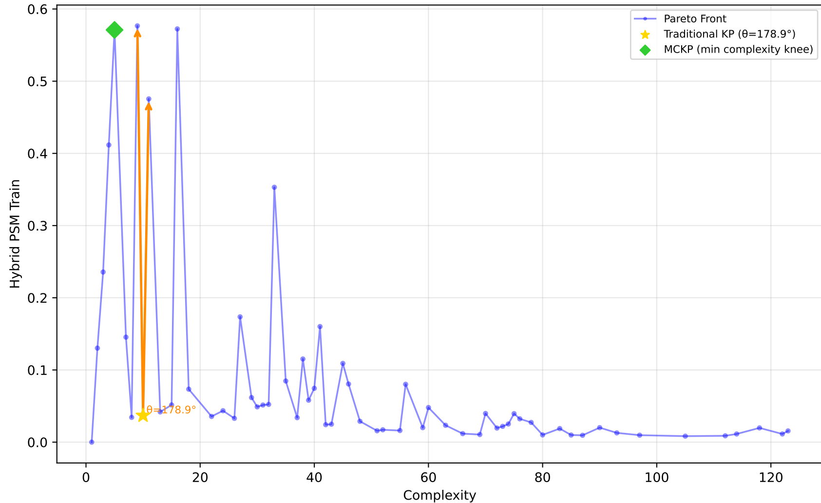
584_fri_c4_500_25 - Run 13 - SVP - Hybrid PSM Train \lambda_1=0.10, \lambda_2=0.40, \lambda_3=0.00 | Difficulty: 1.00 | Method: hmr
