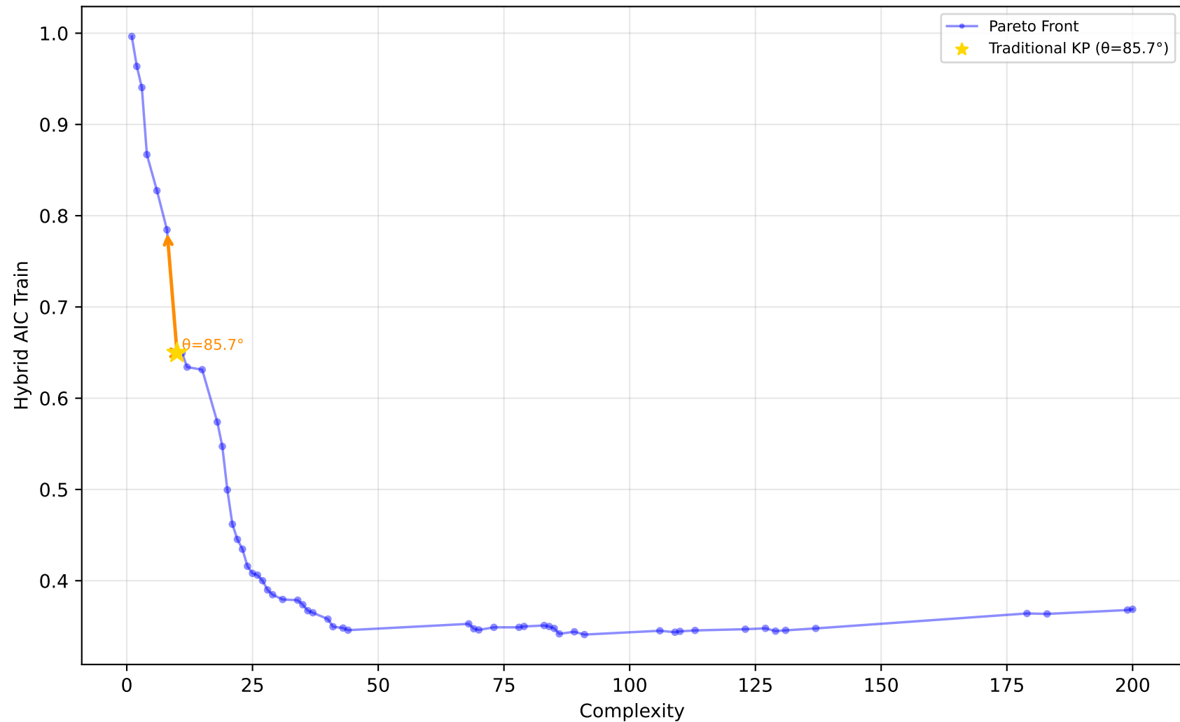
584_fri_c4_500_25 - Run 14 - MVP - Hybrid AIC Train \lambda_1=0.10, \lambda_2=0.00, \lambda_3=0.00 | Difficulty: 1.00 | Method: hmr
