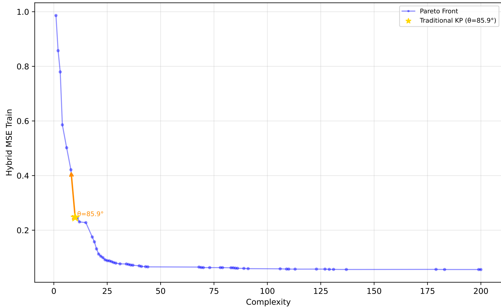
584_fri_c4_500_25 - Run 14 - MVP - Hybrid MSE Train \lambda_1=0.10, \bar{\lambda}_2=0.00, \bar{\lambda}_3=0.00 | Difficulty: 1.00 | Method: hmr
