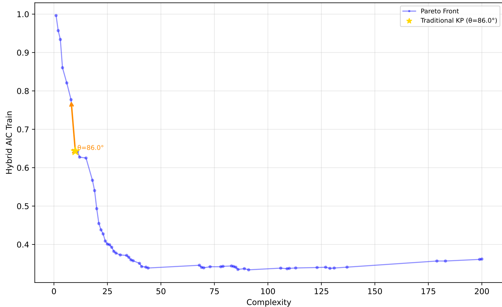
584_fri_c4_500_25 - Run 14 - SVP - Hybrid AIC Train \lambda_1=0.00 , \lambda_2=0.00 , \lambda_3=0.00 | Difficulty: 1.00 | Method: hmr
