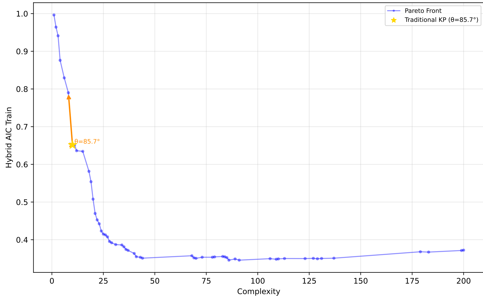
584_fri_c4_500_25 - Run 14 - SVP - Hybrid AIC Train \lambda_1=0.10 , \lambda_2=0.40 , \lambda_3=0.00 | Difficulty: 1.00 | Method: hmr
