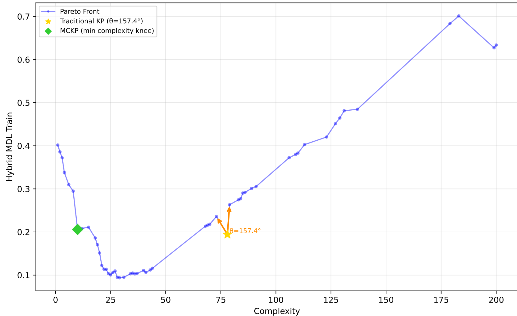
584_fri_c4_500_25 - Run 14 - SVP - Hybrid MDL Train \lambda_1=0.10, \lambda_2=0.40, \lambda_3=0.00 | Difficulty: 1.00 | Method: hmr
