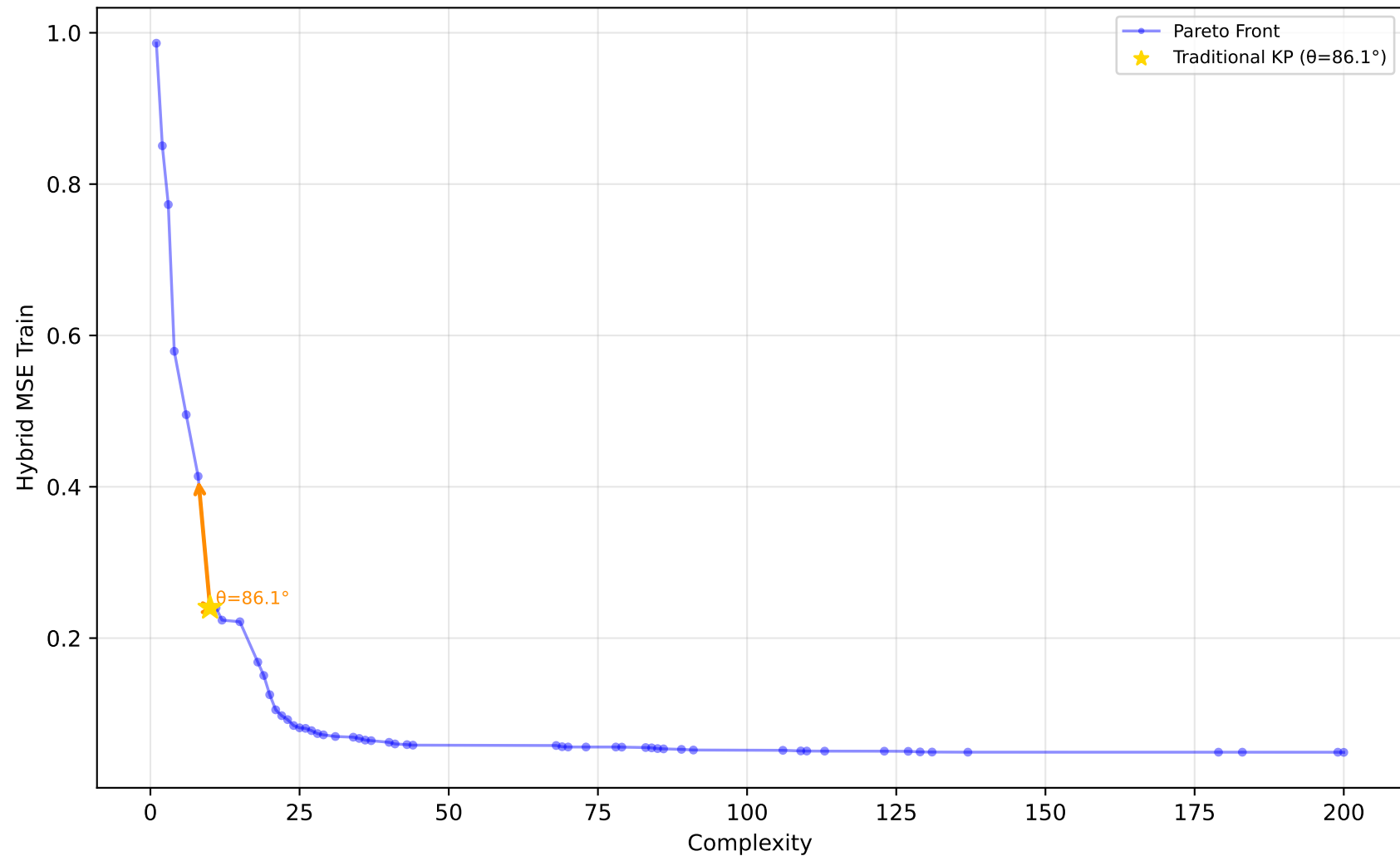
584_fri_c4_500_25 - Run 14 - SVP - Hybrid MSE Train \lambda_1=0.00, \lambda_2=0.00, \lambda_3=0.00 | Difficulty: 1.00 | Method: hmr
