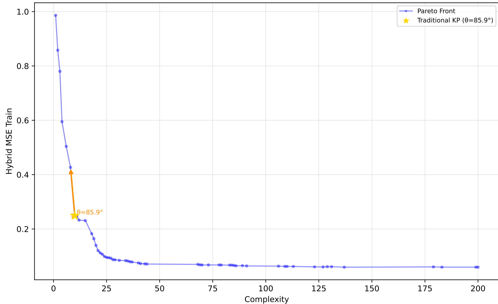
584_fri_c4_500_25 - Run 14 - SVP - Hybrid MSE Train \lambda_1=0.10, \lambda_2=0.40, \lambda_3=0.00 | Difficulty: 1.00 | Method: hmr
