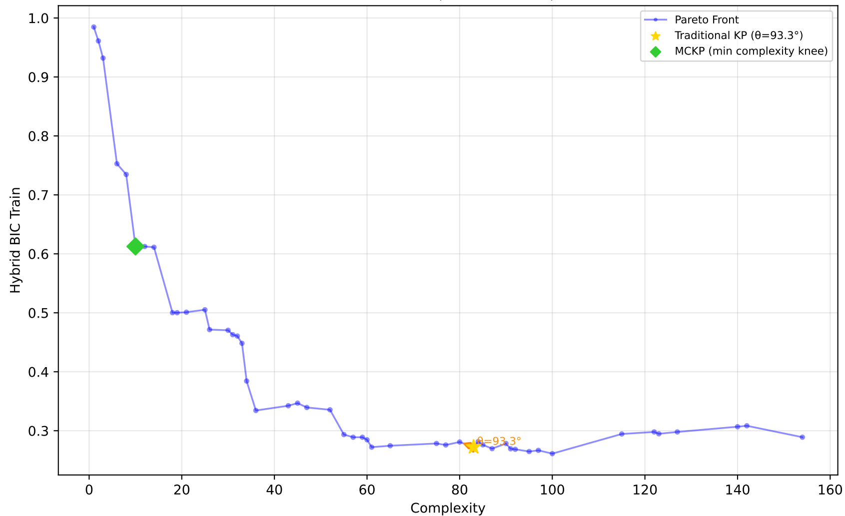
584_fri_c4_500_25 - Run 15 - MVP - Hybrid BIC Train \lambda_1=0.00, \lambda_2=0.00, \lambda_3=0.00 | Difficulty: 1.00 | Method: hmr
