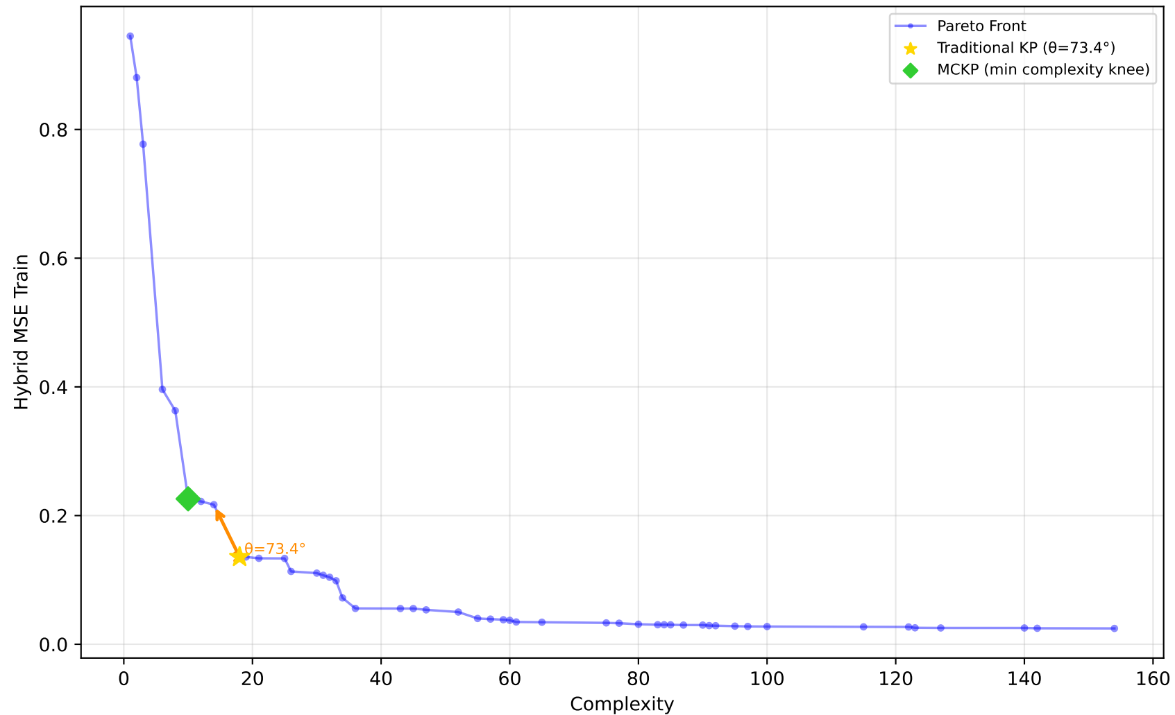
584_fri_c4_500_25 - Run 15 - MVP - Hybrid MSE Train \lambda_1=0.00, \lambda_2=0.00, \lambda_3=0.00 | Difficulty: 1.00 | Method: hmr
