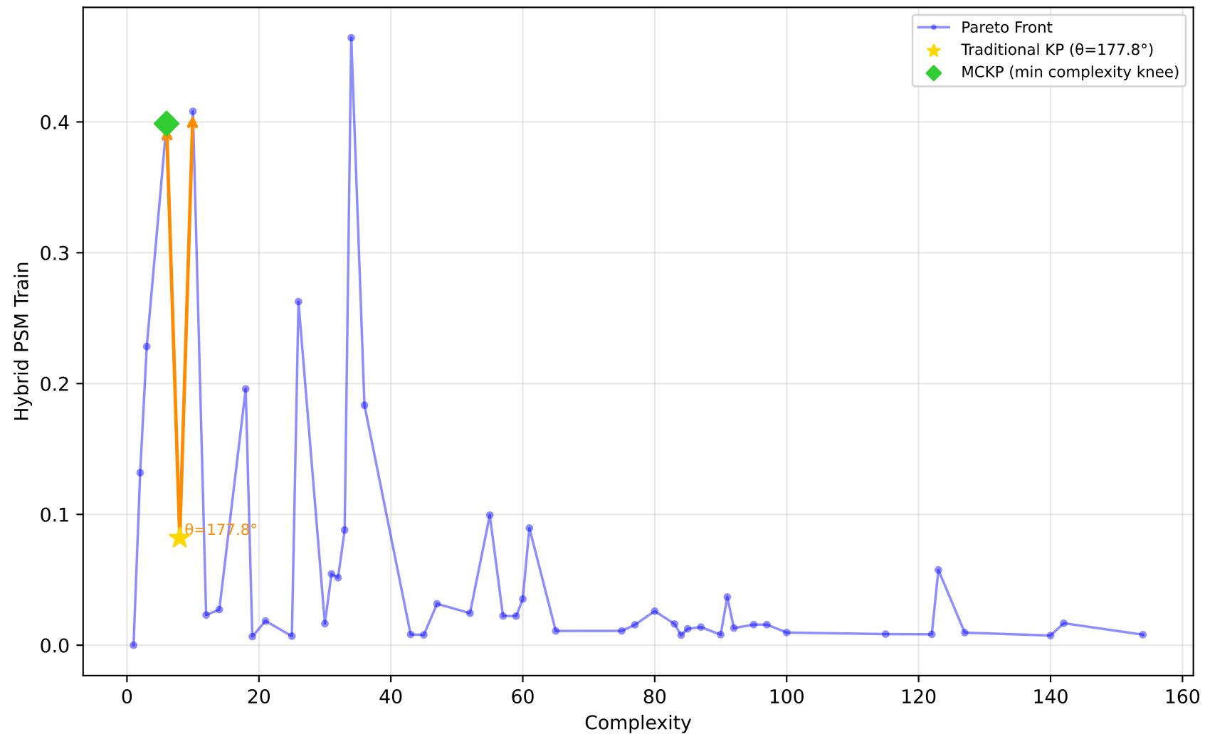
584_fri_c4_500_25 - Run 15 - MVP - Hybrid PSM Train \lambda_1=0.10, \lambda_2=0.00, \lambda_3=0.00 | Difficulty: 1.00 | Method: hmr
