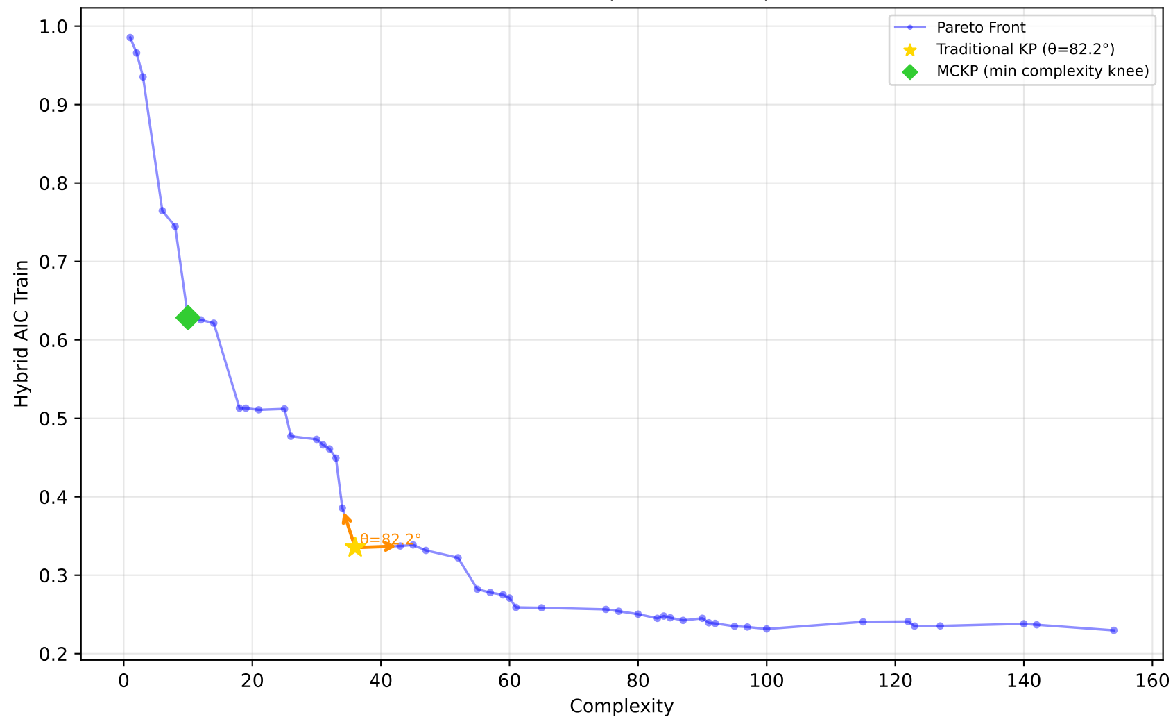
584_fri_c4_500_25 - Run 15 - SVP - Hybrid AIC Train \lambda_1=0.00, \lambda_2=0.00, \lambda_3=0.00 | Difficulty: 1.00 | Method: hmr
