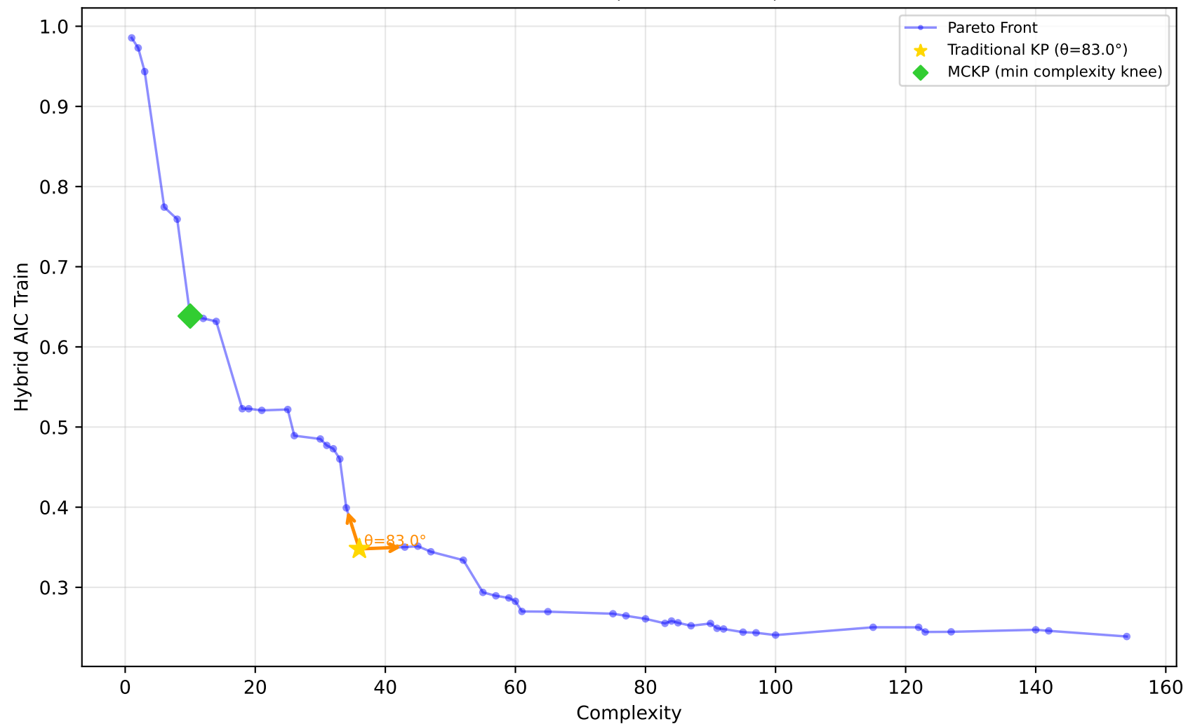
584_fri_c4_500_25 - Run 15 - SVP - Hybrid AIC Train \lambda_1=0.10, \lambda_2=0.40, \lambda_3=0.00 | Difficulty: 1.00 | Method: hmr
